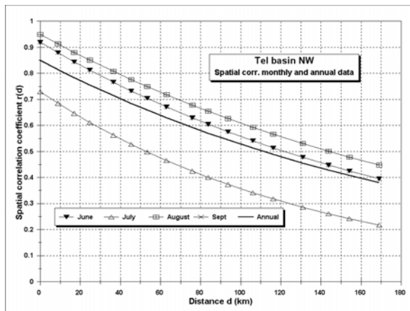
Figure 1.19: r(d) for monthly and annual data, Tel NW basin
